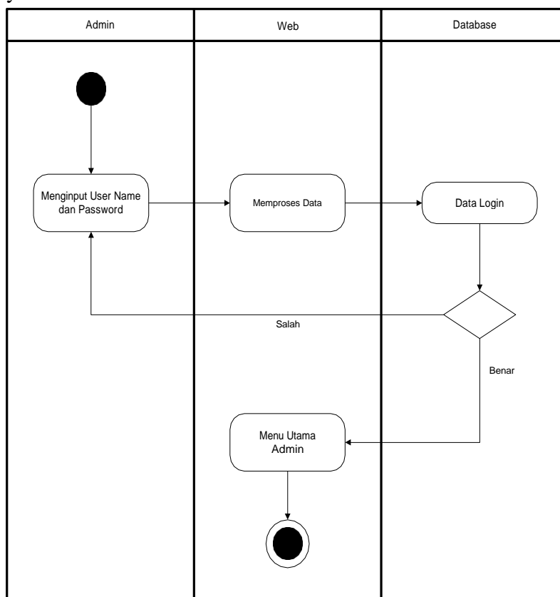
Gambar 2. Activity Diagram
