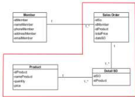
Gambar 2.16 contoh class diagram
